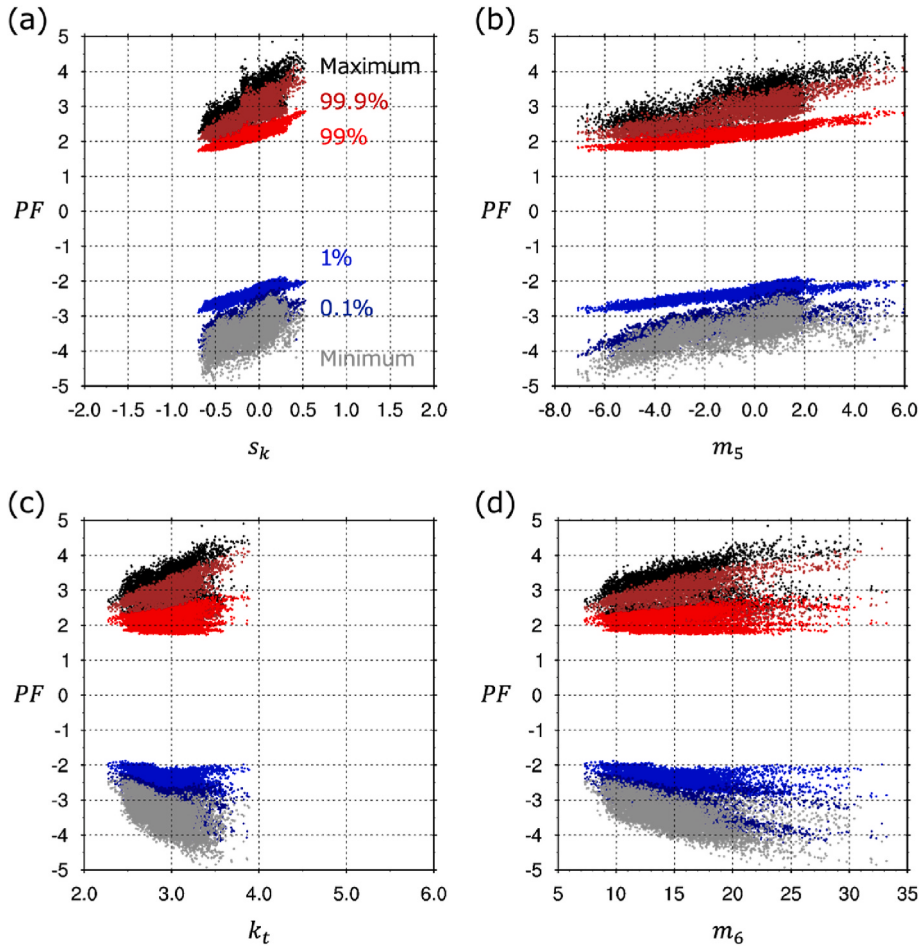
Fig. 8. Relationship between the peak factor and higher-order statistics of the streamwise velocity component u at z/H = 0.5 . (a) Skewness, (b) fifth-order moment, (c) kurtosis, and (d) sixth-order moment. The maximum (99.9th and 99th) percentiles represent strong wind speed events, whereas the minimum (0.1st and 1st) percentiles indicate the weak-wind-speed events.
