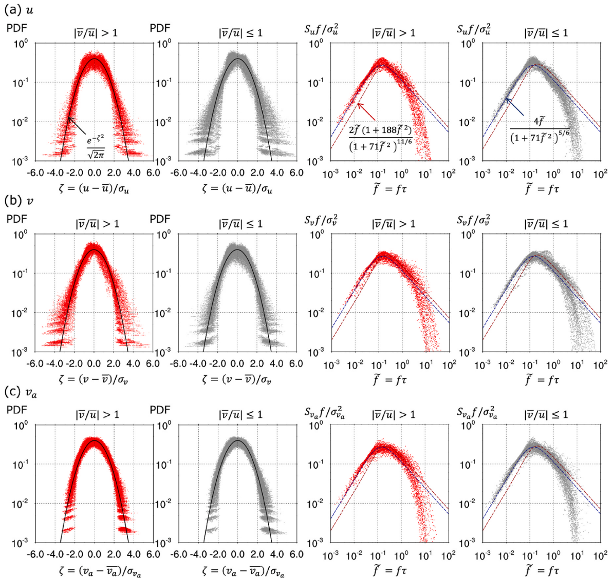
Fig. 6. The relationship between probability density functions, PDFs, and power spectral densities, PSDs, S_{u_i} , by two-class categorization of the spanwise-dominated ( |\bar{v}/\bar{u}| > 1 ) and streamwise-dominated ( |\bar{v}/\bar{u}| \leq 1 ) flow regions for (a) the streamwise velocity component u , (b) spanwise velocity component v , and (c) wind speed v_a .
